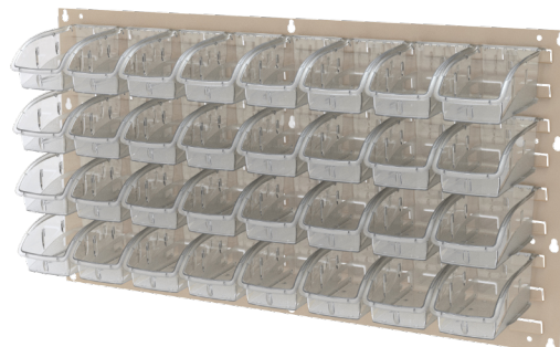
Louvered panel 30636 shown with 305A3 bins
